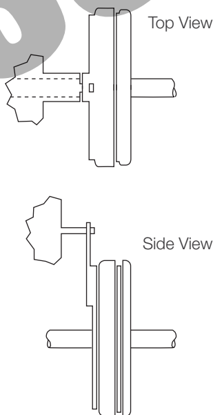
Figure 3: Pin in Hole Loosely (Preferred)
