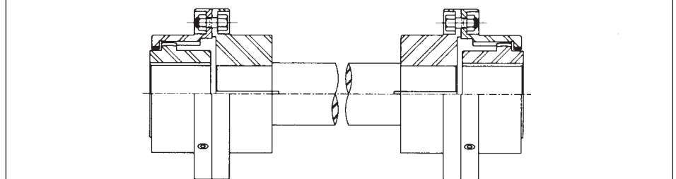
FIG. B TANDEM - RIGID HALVES ON FLOATING SHAFT
