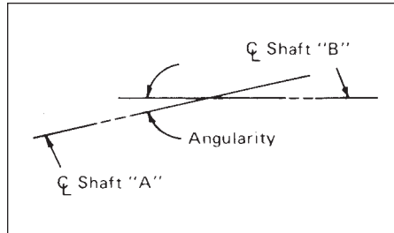
Figure 1 — Angularity is the acute angle formed at the intersection of the axes of the driving and the driven machine shafts. When shafts are exactly parallel, angular misalignment is zero; but vertical or horizontal displacement of axes may be present (See Fig. 2).
