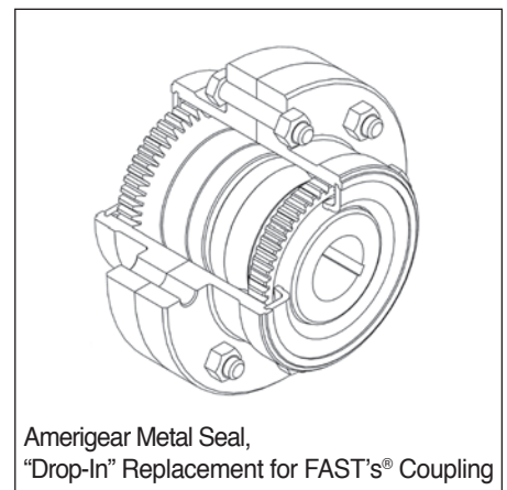
Amerigear Series C Continuous Sleeve Flexible Coupling
