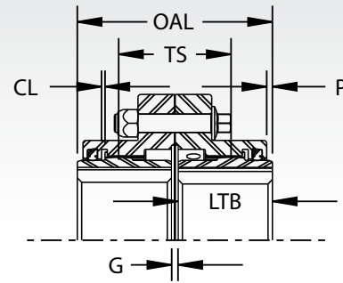
Normal Hub Arrangement
