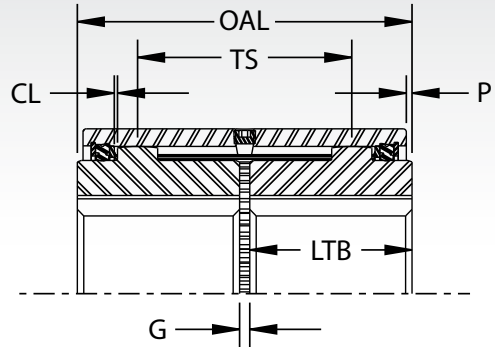
Normal Hub Arrangement
